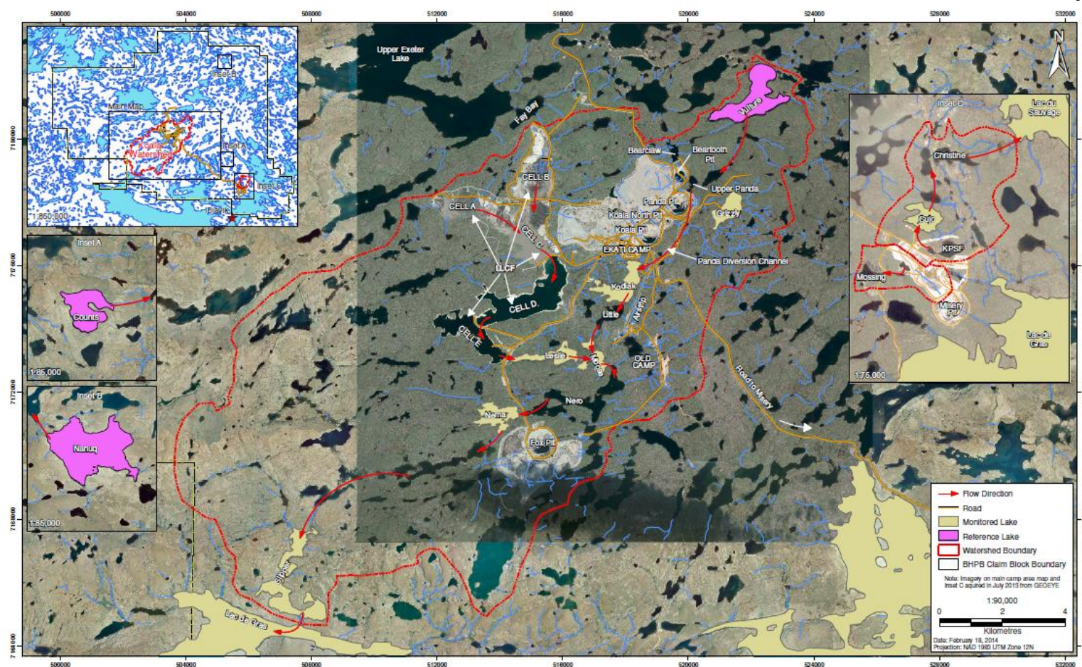
Figure 2: Surface water flow through the AEMP sampling area from Ekati Diamond Mine 2013 Aquatic Effects Monitoring Program Summary Report March 2014
